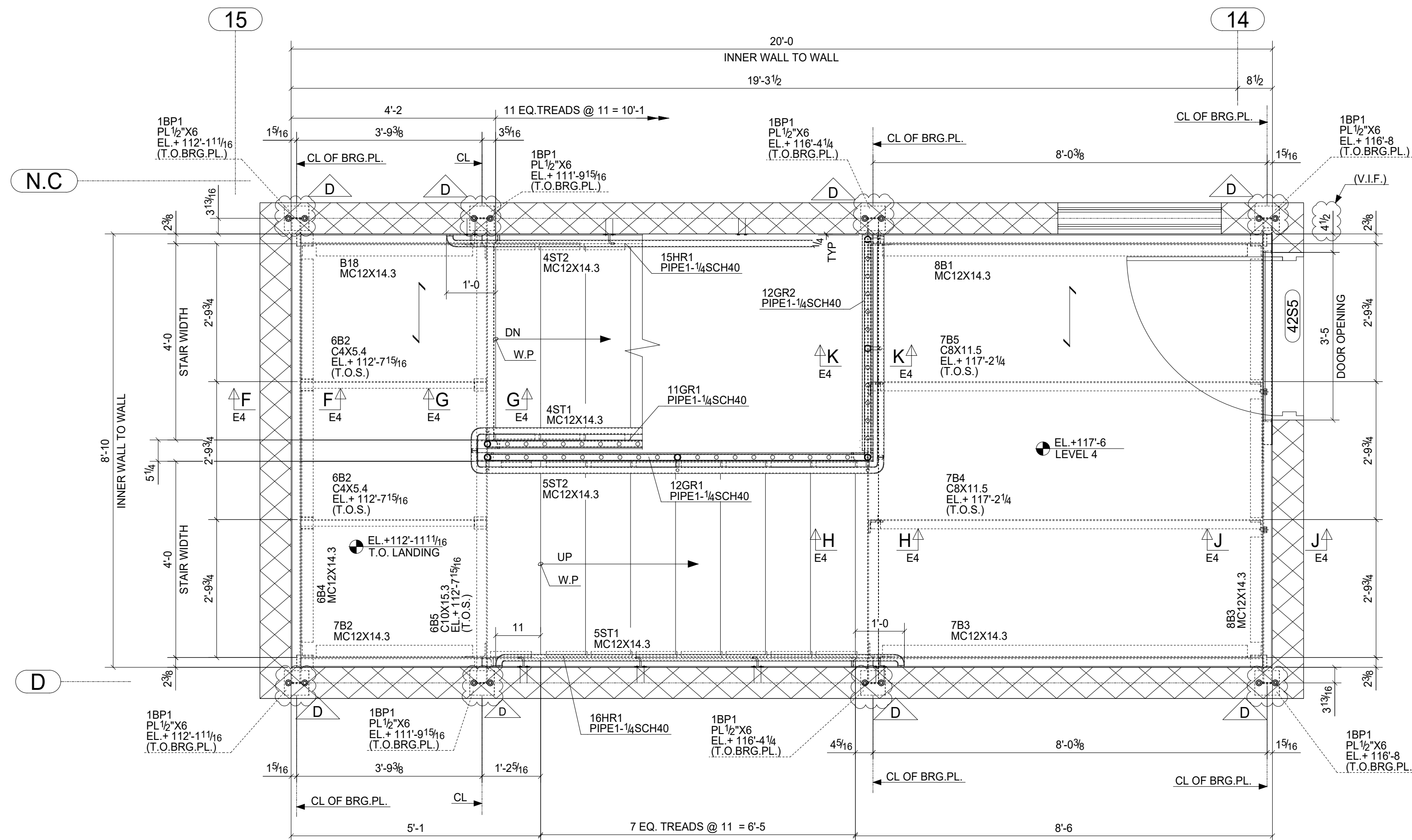
STAIR 11 MARKING PLAN AT LEVEL 3 (REF. CONTRACT DWG. NO. - 3/A0860)
