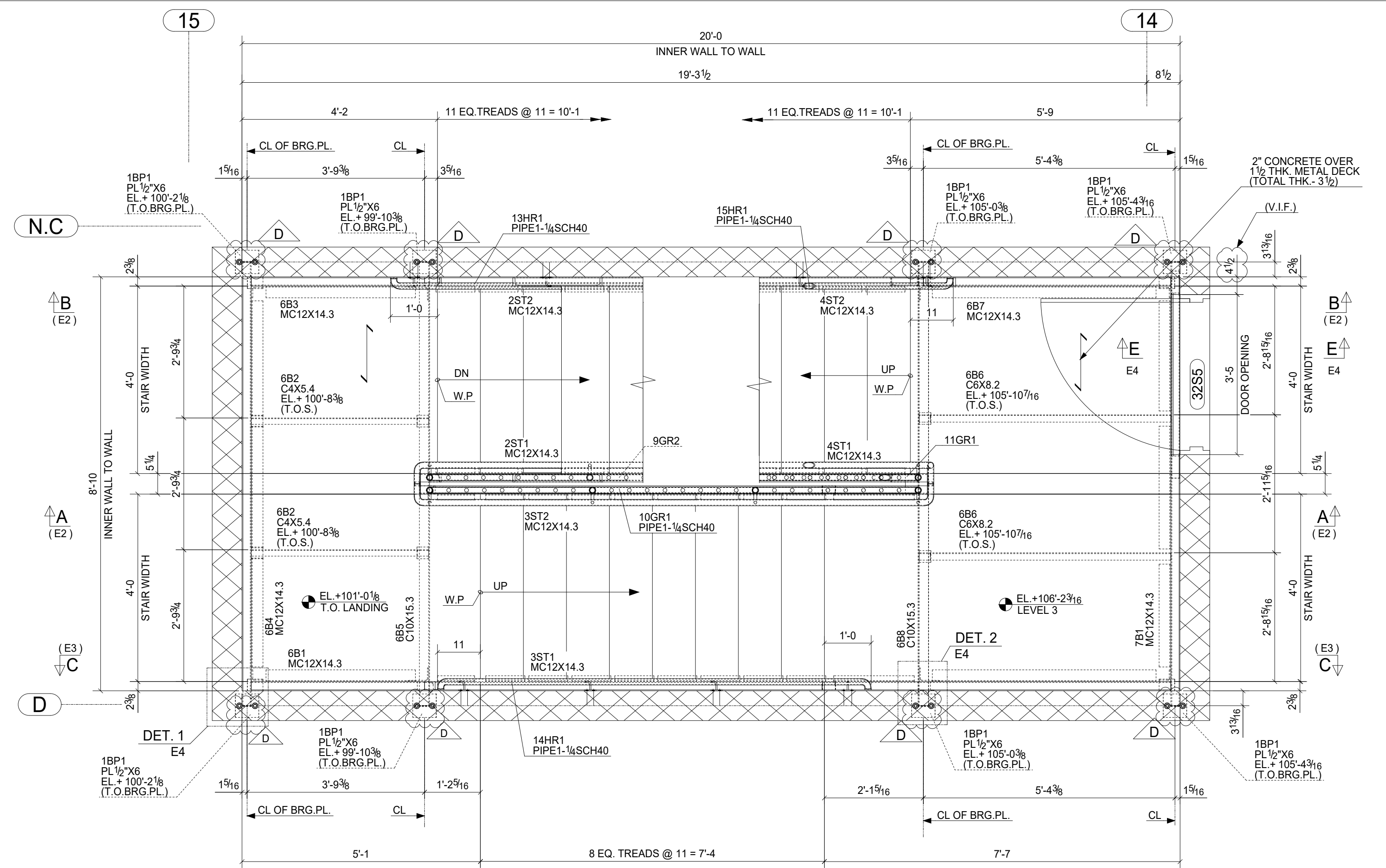
STAIR 1 MARKING PLAN AT LEVEL 2 (REF. CONTRACT DWG. NO. - 2/A0860)
